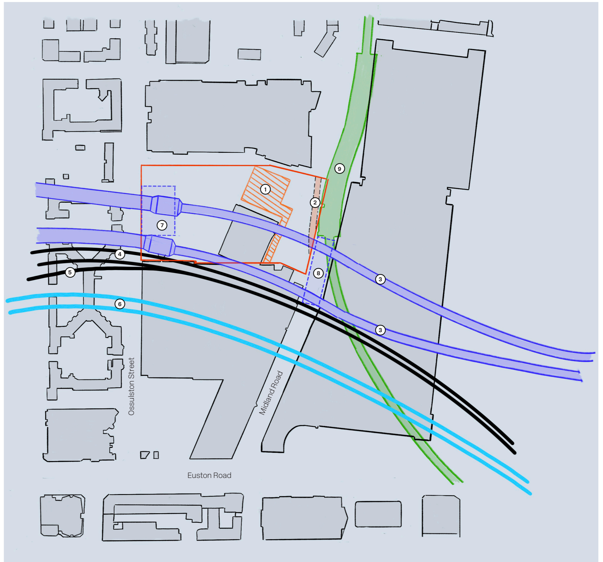
SITE CONSTRAINTS: PLAN BELOW GROUND LEVEL
